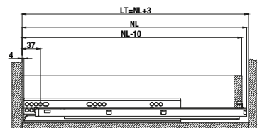
Cajón Interior Internal drawer
