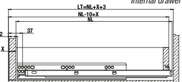
Cajón Interior Internal drawer
