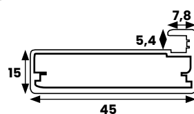
Perfl perimetral (TIR/PEL)
